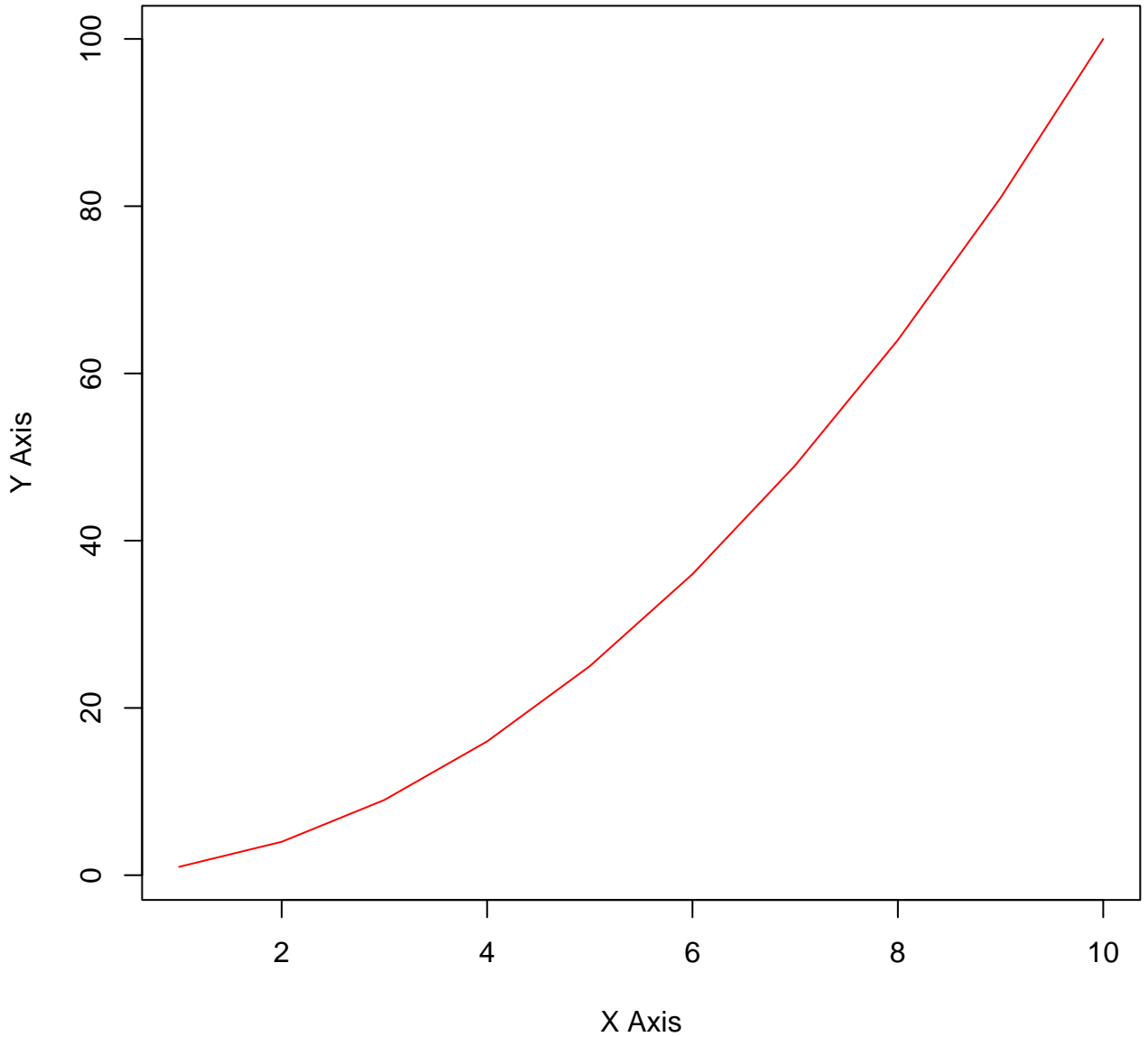
Line Plot
