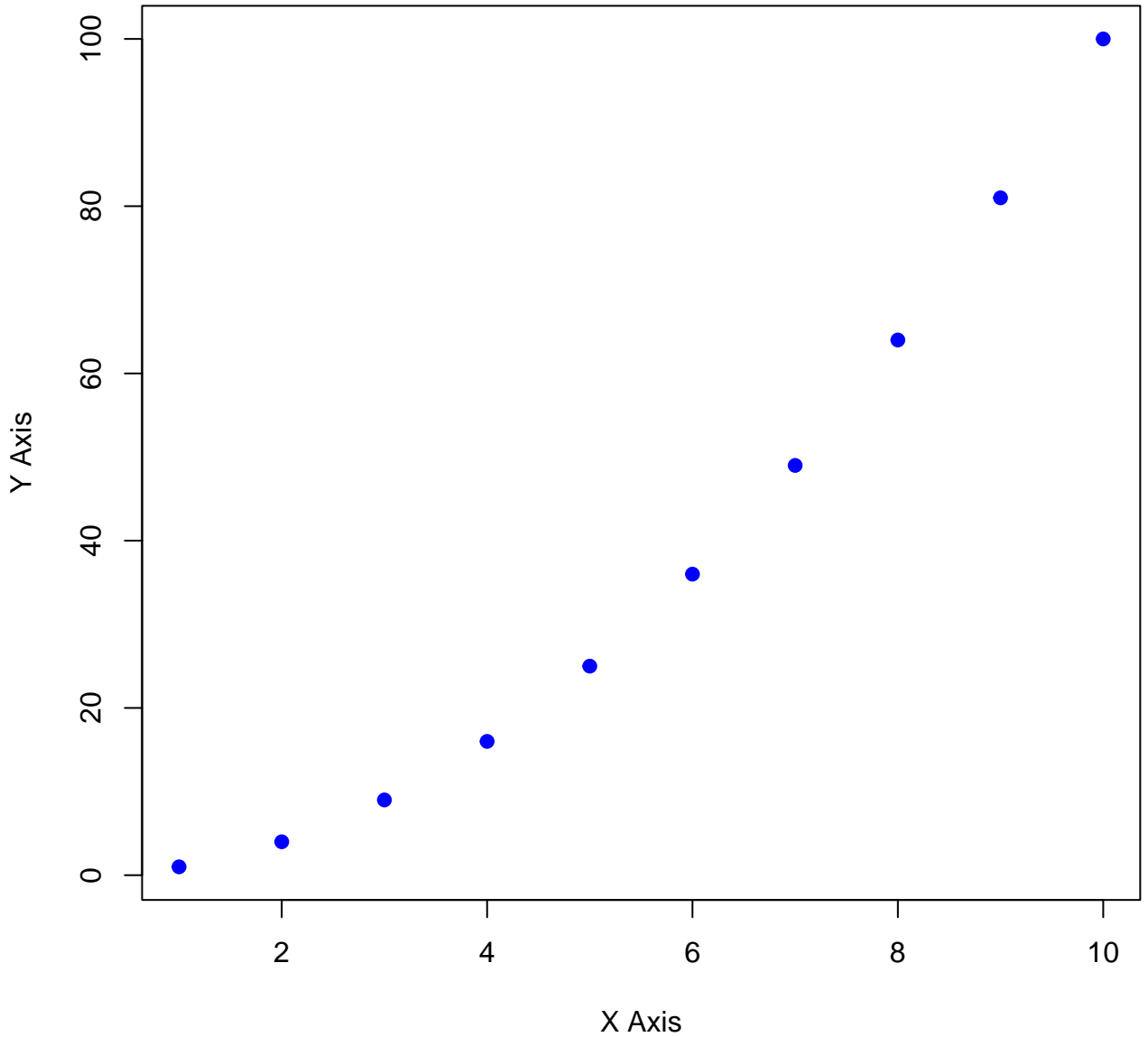
Scatter Plot
